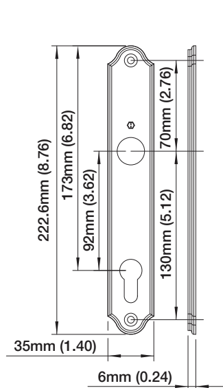
Interior Backplate
