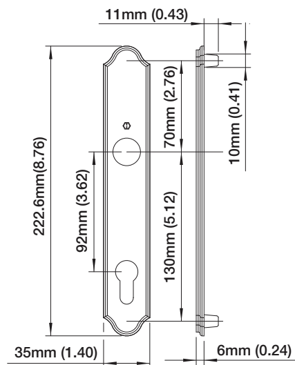
Exterior Backplate
