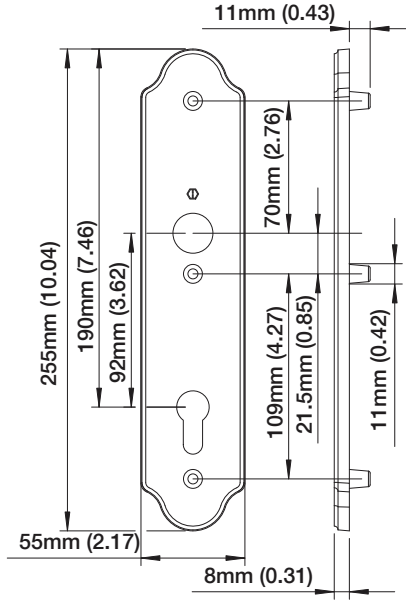
Interior Backplate
