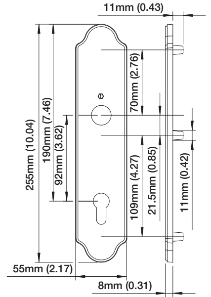
Exterior Backplate
